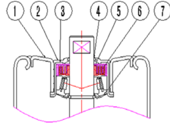
TAPERED BEARING STRUCTURE
