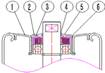
Ball Bearing Structure
