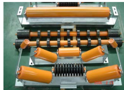
HDPE Idlers with SUS or Anti-Vibration
