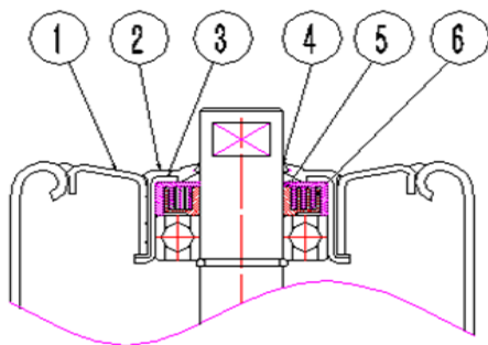
Ball Bearing Structure
