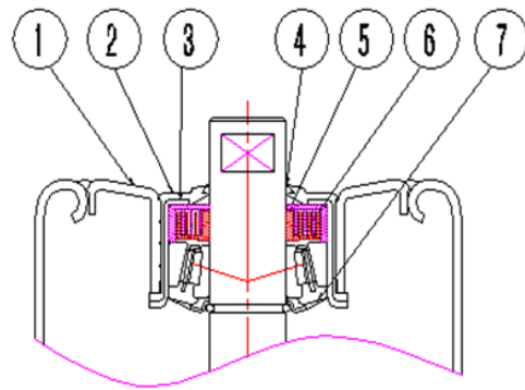
TAPERED BEARING STRUCTURE
